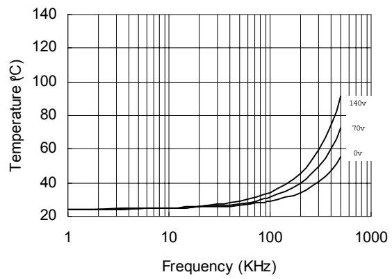
Figure 28. IR21834 vs. Frequency (IRFBC40), R_{gate}=15\Omega , V_{CC}=15V
