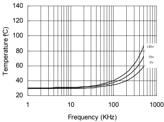
Figure 23. IR2183 vs. Frequency (IRFBC30), R_{gate}=22\Omega, V_{cc}=15V
