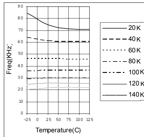
Fig. 14 Frequency vs RFMIN vs TEMP VVCO=6V
