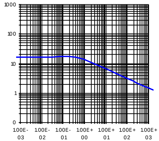
Figure 13 - I_{\text{clamp}} (A) Vs Power Supply Wire Inductance (mH - single pulse)
