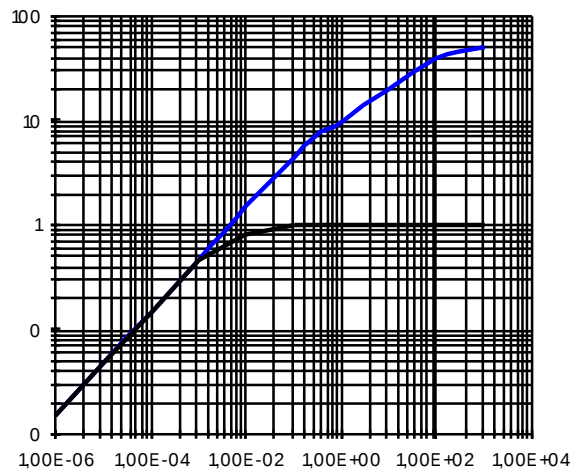
Figure 12 - Transient Thermal Imped. ( ^{\circ}\text{C/W} ) Vs Time (S)
