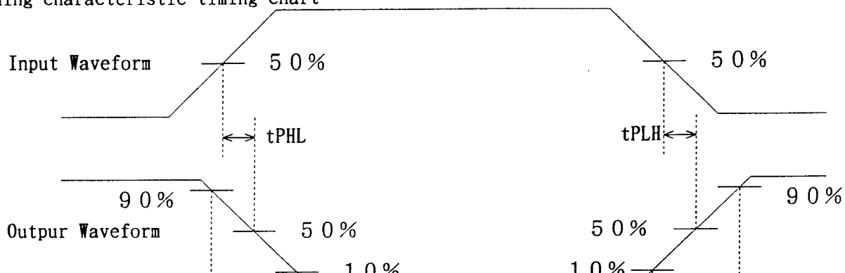
Switching characteristic timing chart
