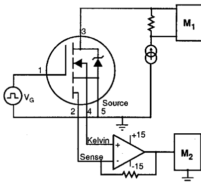
Fig 18. HEXSense Ratio Test Circuit
