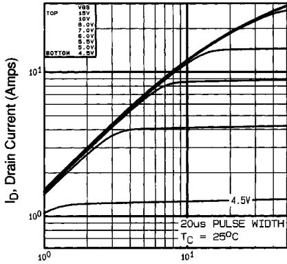
Fig 1. Typical Output Characteristics, T_C=25^\circ\text{C}
