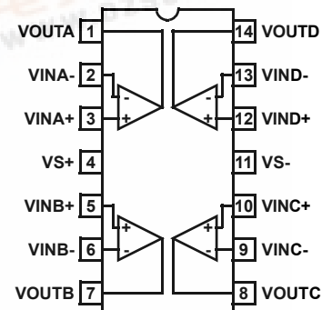
EL5411 (14-PIN HTSSOP) TOP VIEW
