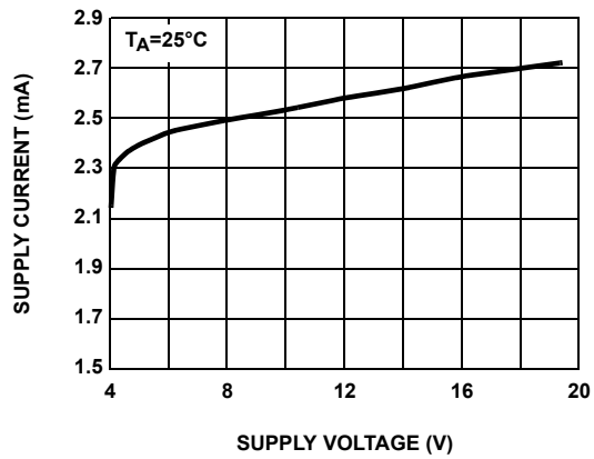
FIGURE 9. SUPPLY CURRENT PER AMPLIFIER vs SUPPLY VOLTAGE
