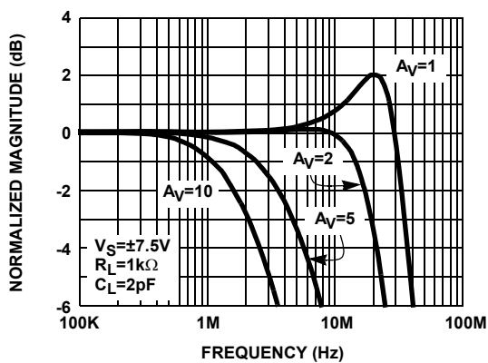
FIGURE 10. FREQUENCY RESPONSE ( V_{COM} )
