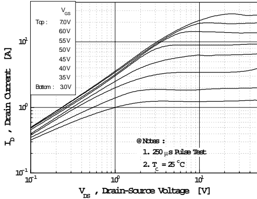
Fig 1. Output Characteristics
