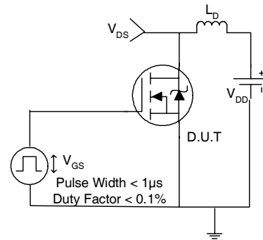
Fig 10a. Switching Time Test Circuit
