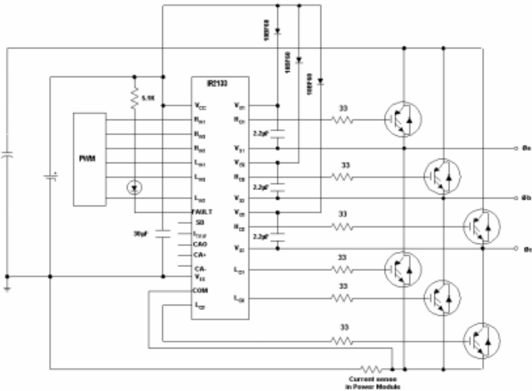
Figure 10. Recommended Gate Drive Circuit
