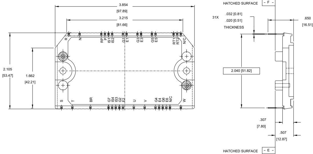
Figure 8a. Package Outline and Mechanical Specifications
