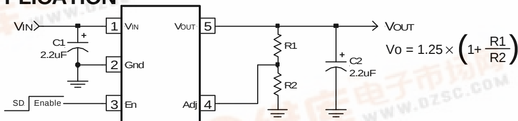
Figure 1 - Typical application of the IRU1205 ajustable voltage regulator.
