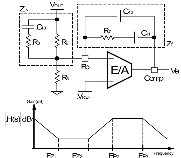
Figure 7 - Compensation network with local feedback and its asymptotic gain plot.
