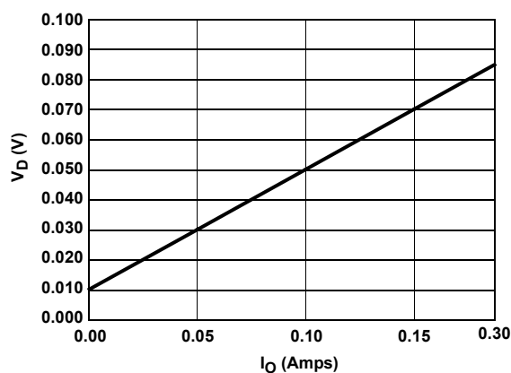
FIGURE 2. LD03 DROPOUT VOLTAGE
