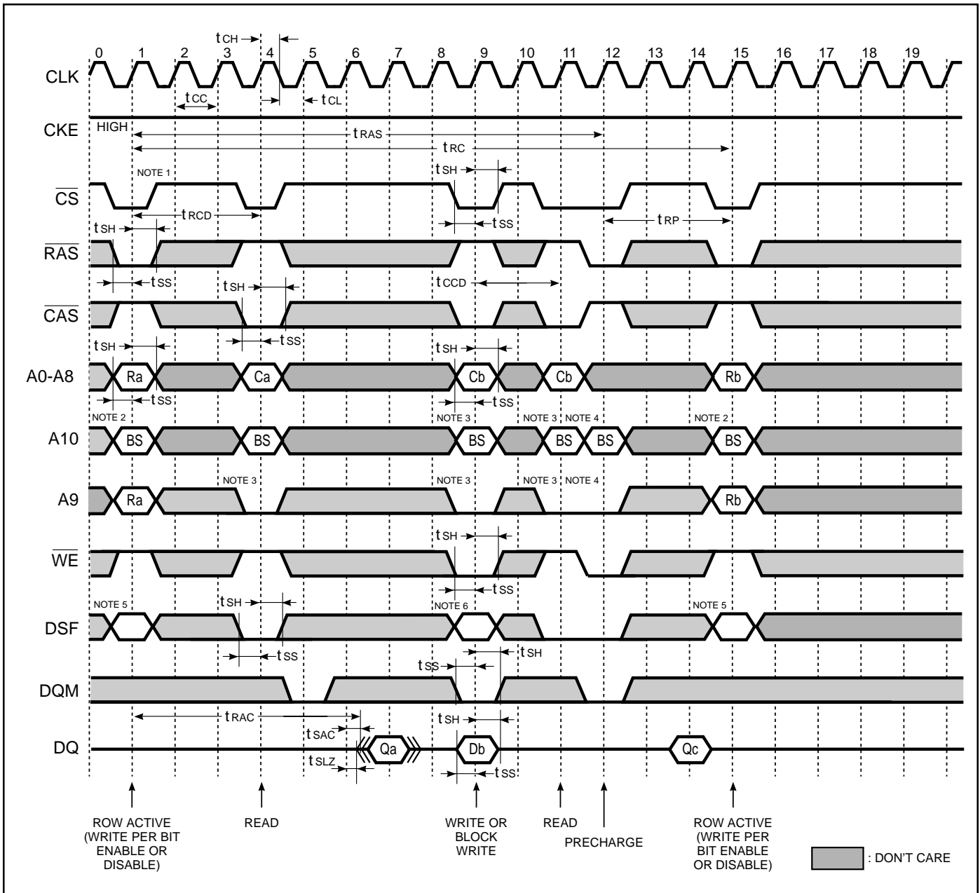
Figure 19. Single Bit Read-Write-Read Cycle (Same Page) at \overline{CAS} Latency = 3, Burst Length = 1
