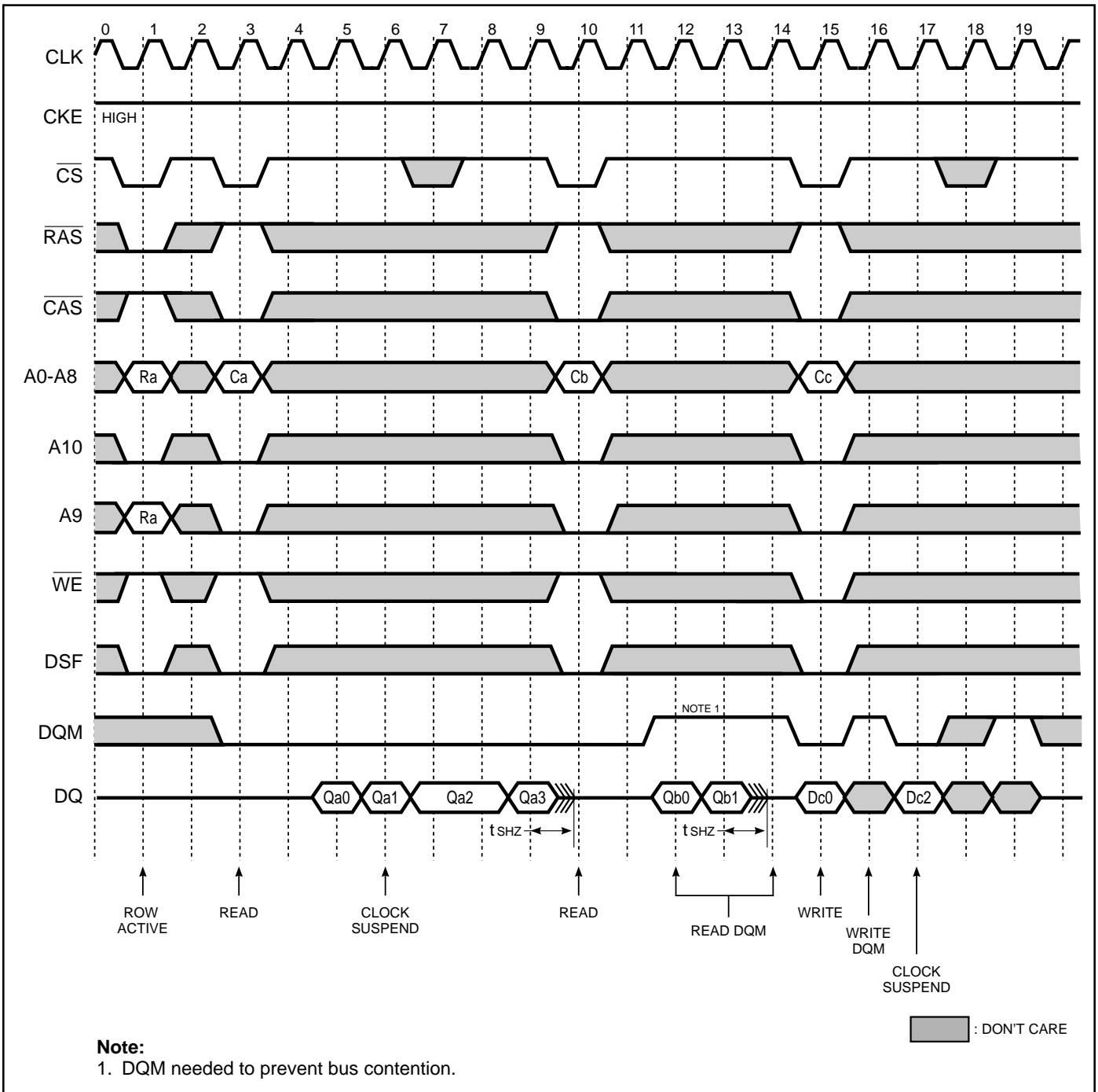
Figure 33. Clock Suspension and DQM Operation Cycle at CAS Latency = 2, Burst Length = 4
