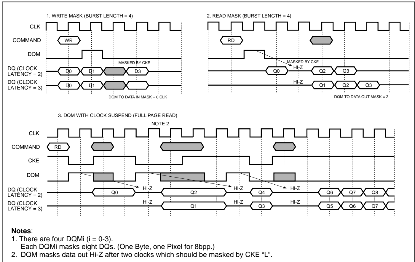
Figure 5. DQM Operation
