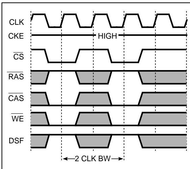
Figure 3. Timing Diagram to Illustrate t_{BWC} . (2CLK Cicle Block Write)
