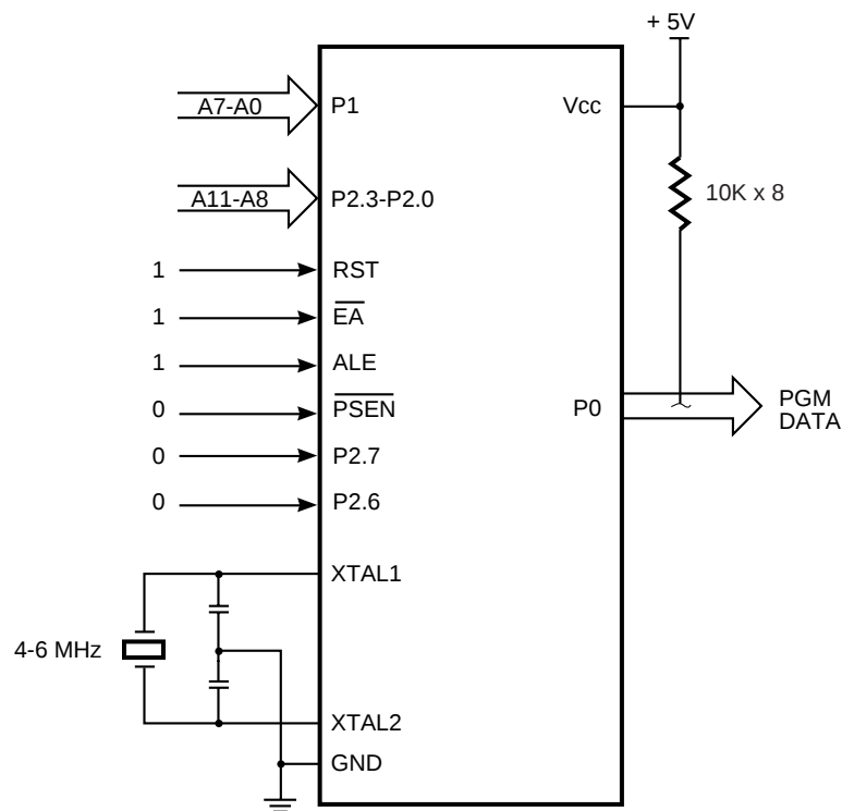
Figure 24. ROM Verification
