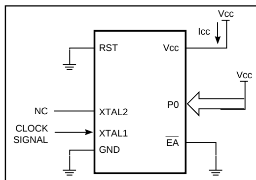
Figure 26. Idle Mode
