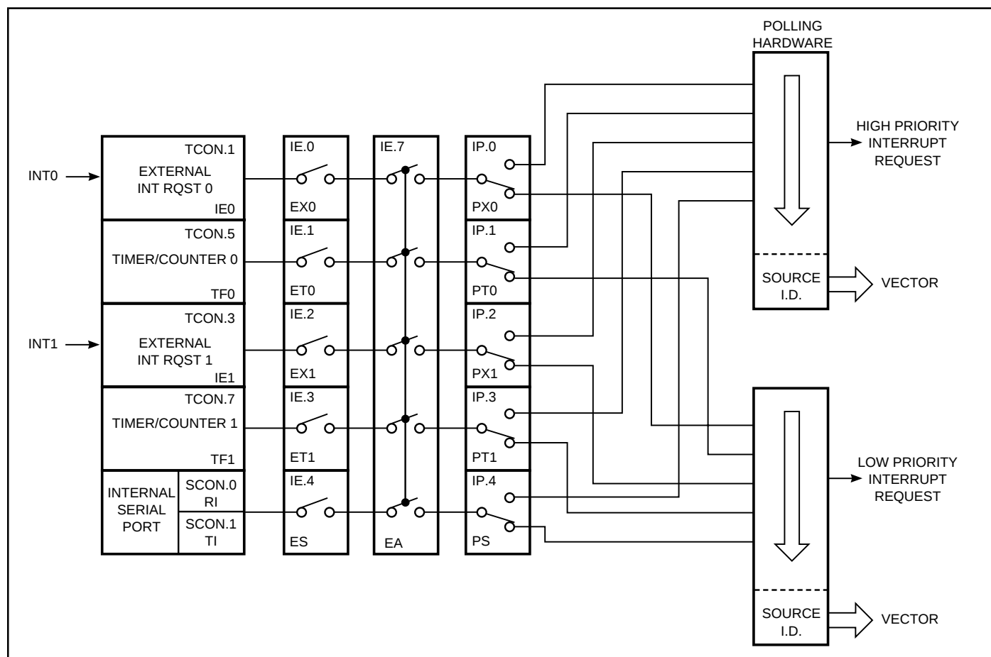
Figure 16. Interrupt System
