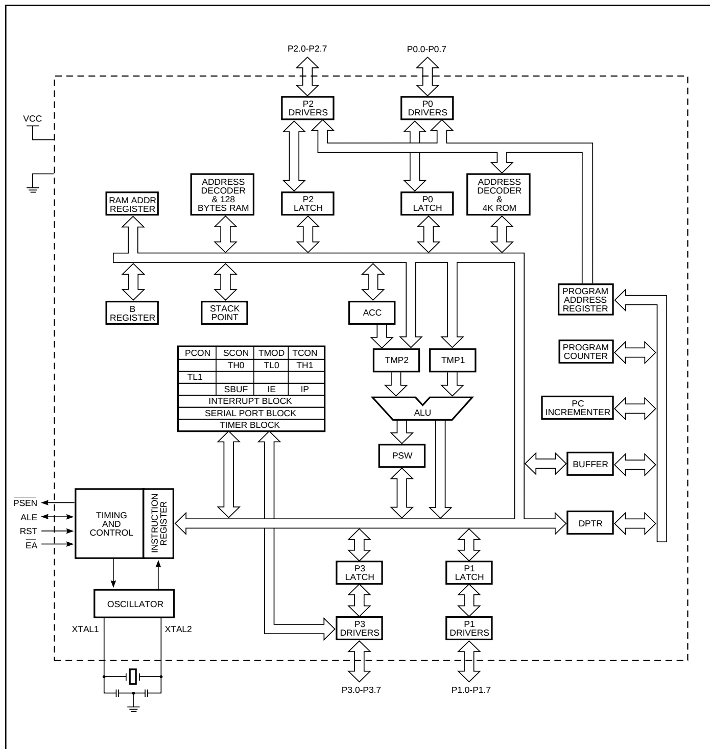
Figure 4. IS80C51/31 Block Diagram
