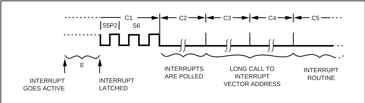
Figure 17. Interrupt Response Timing Diagram
