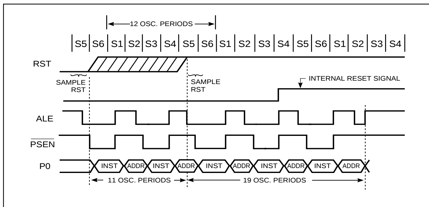
Figure 18. Reset Timing
