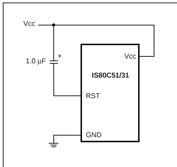
Figure 19. Power-On Reset Circuit
