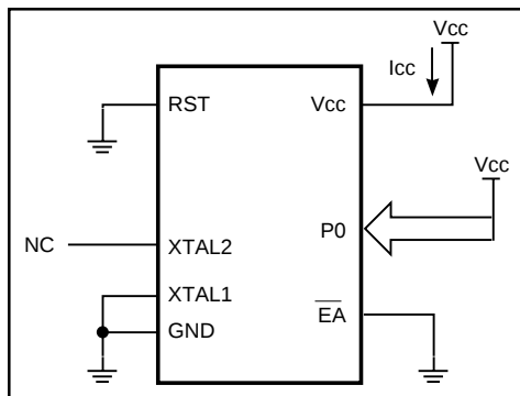
Figure 27. Power-down Mode
