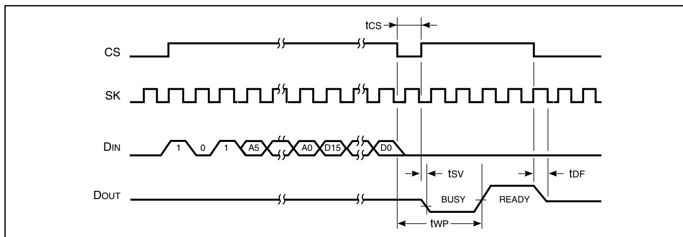
FIGURE 5. WRITE (WRITE) CYCLE TIMING
