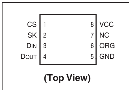
8-pad DFN
