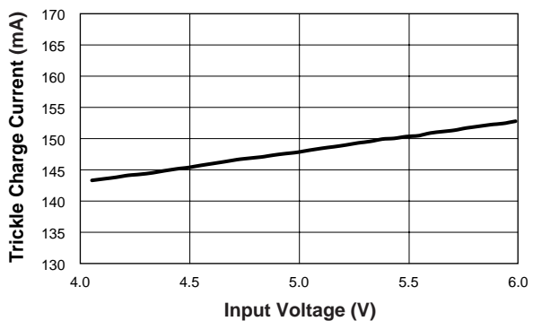
Trickle Charge Current vs. Input Voltage ( R_{\text{SENSE}} = 0.15\Omega ; 1.8X Mode)
