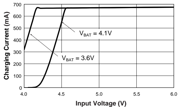
Charging Current vs. Input Voltage ( R_{\text{SENSE}} = 0.15\Omega with External Schottky)
