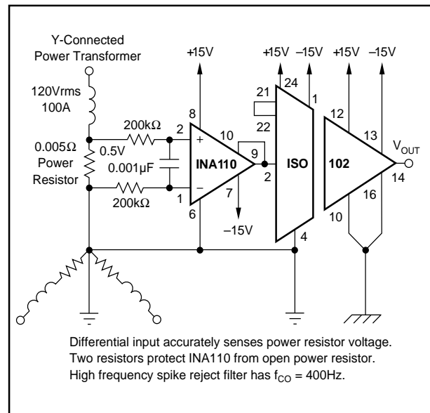
FIGURE 6. Isolated Power Line Monitor ( 0.5\mu\text{A} leakage current at 120Vrms).
