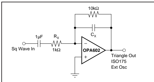
FIGURE 2. Square-Wave to Triangle Wave Signal Conditioner for Driving ISO175 Ext Osc Pin.
