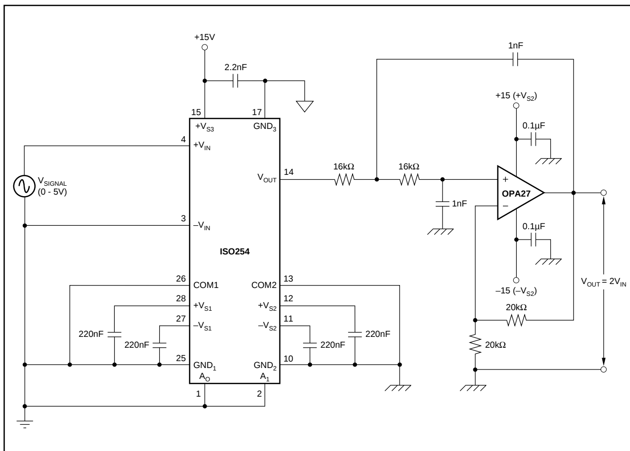
FIGURE 3. Noise Reduction in Data Acquisition System.
