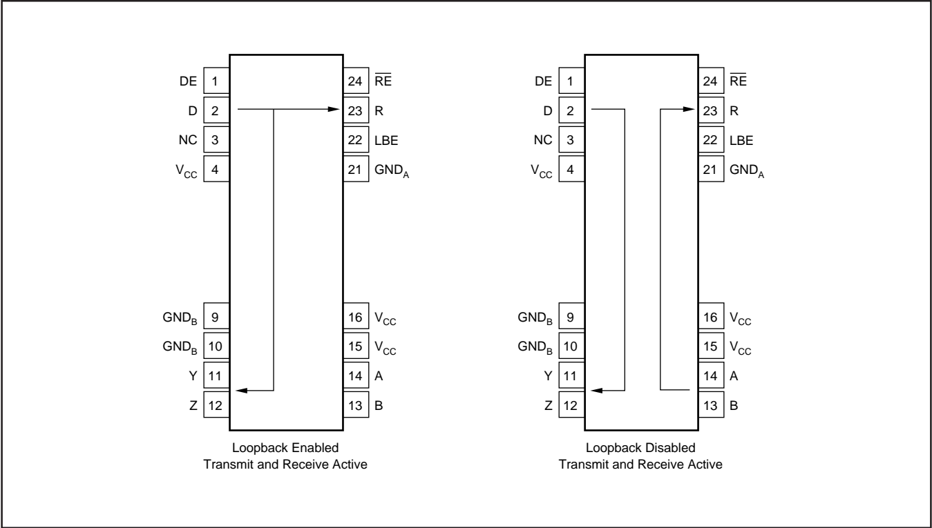
FIGURE 3. Loopback.
