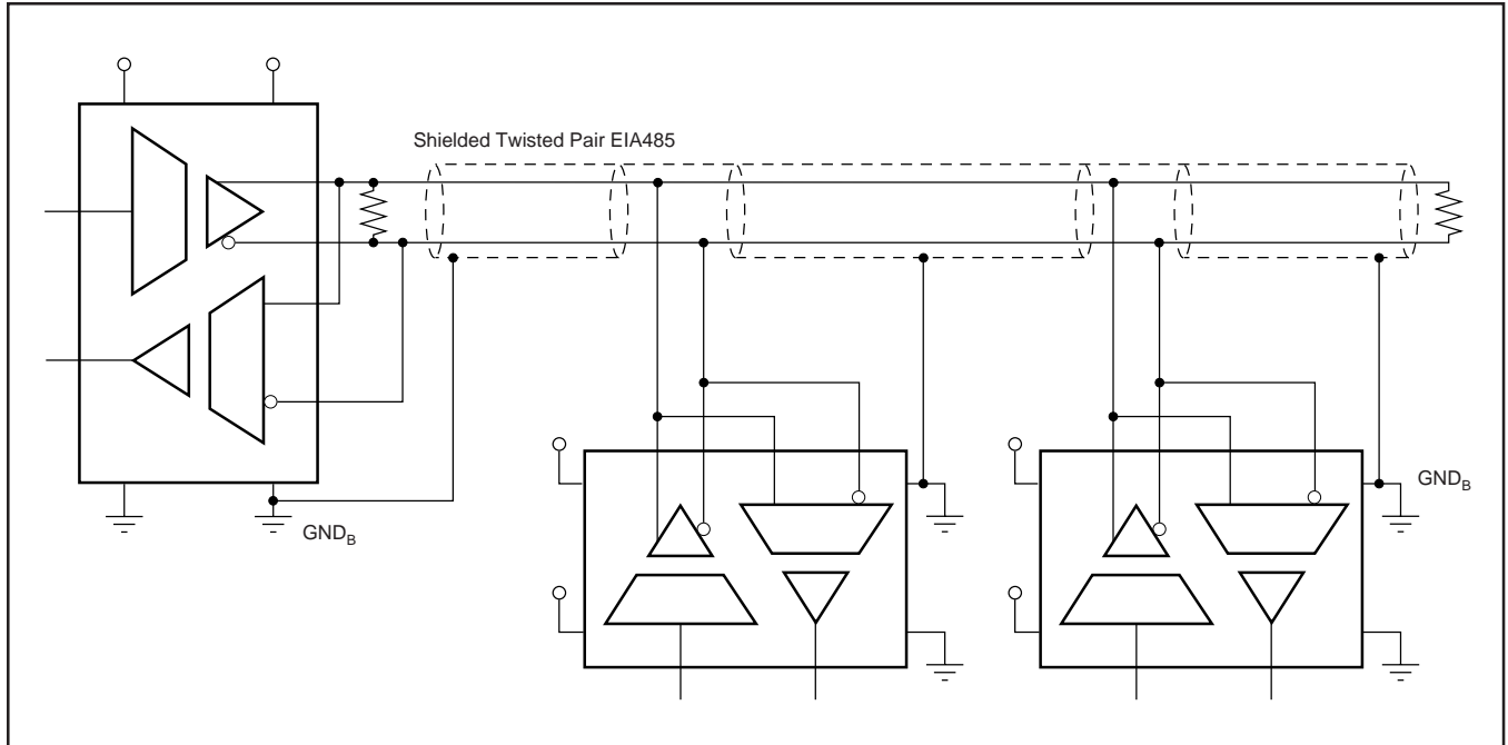
FIGURE 5. Half-Duplex Connection.
