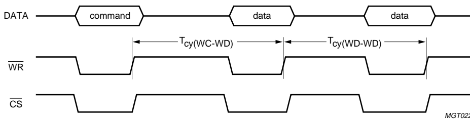
Fig 25. Write command + write data cycle timing.
