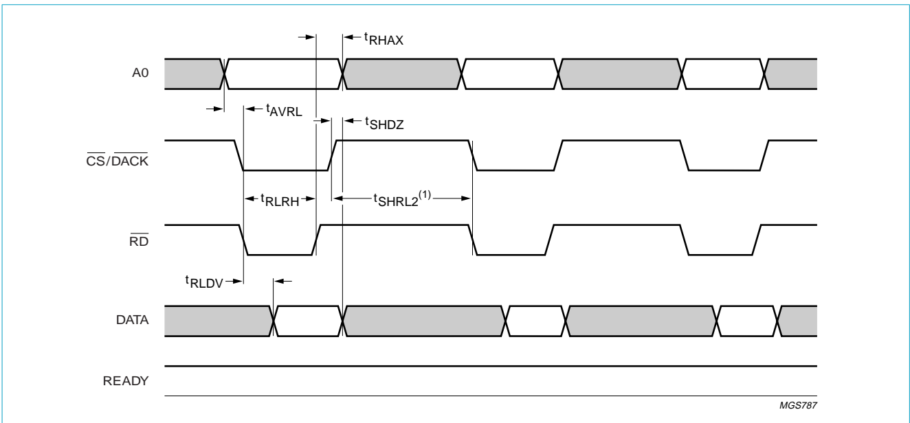
Fig 21. Parallel interface read timing (I/O and 8237 compatible DMA) without READY.
