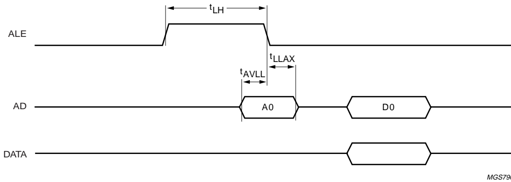
Fig 24. ALE timing.
