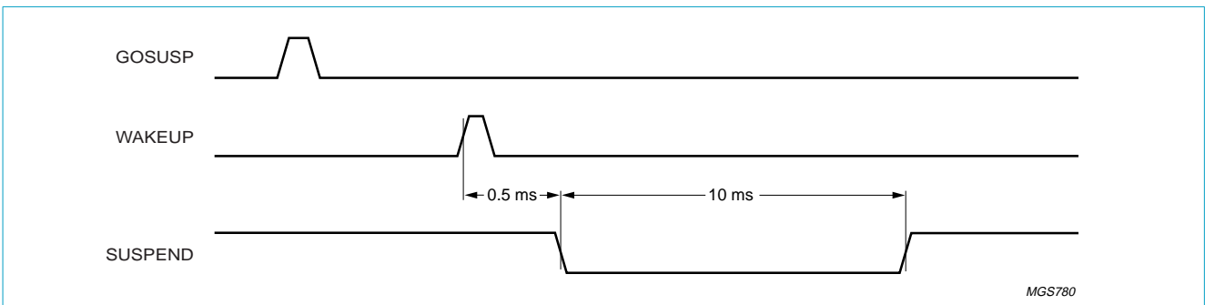
Fig 6. Suspend and resume timing for powered-on application.
