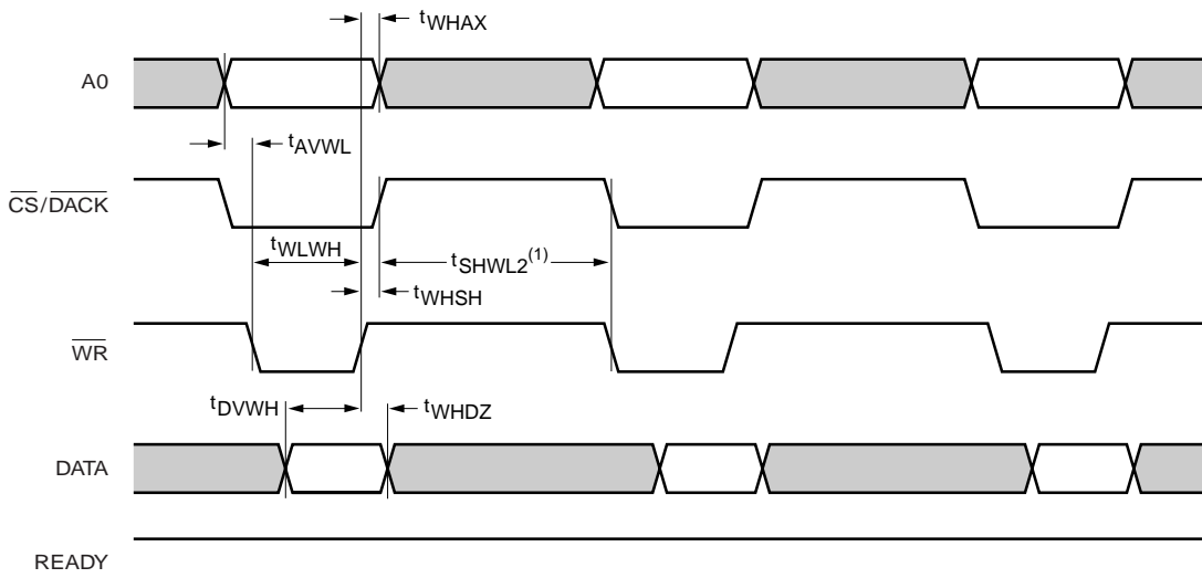
Fig 23. Parallel interface write timing (I/O and 8237 compatible DMA) without READY.
