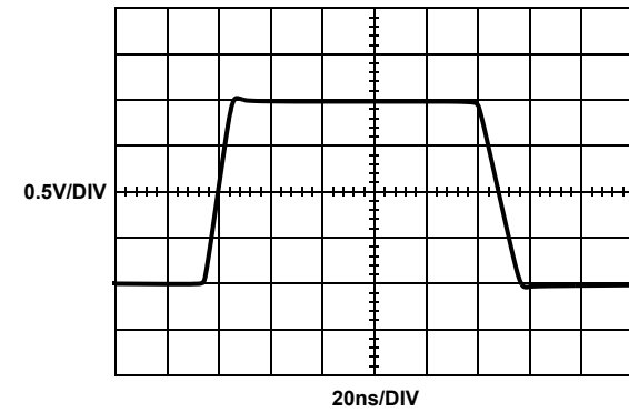
FIGURE 17. V_{COM} TRANSIENT RESPONSE
