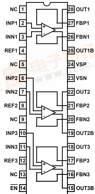
EL5378 (28-PIN QSOP) TOP VIEW
