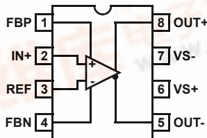
EL5178 (8-PIN MSOP, SO) TOP VIEW
