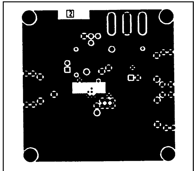
Figure 5. MAX3760 EV Kit PC Board Layout—Ground Plane
