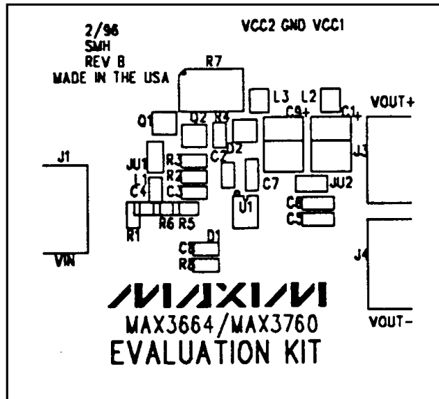
Figure 3. MAX3760 EV Kit Component Placement Guide— Component Side
