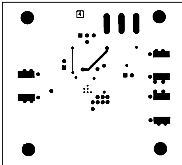
Figure 7. MAX3760 EV Kit PC Board Layout—Solder Side
