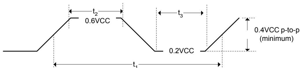
Figure 9-1. LCLK Waveform
