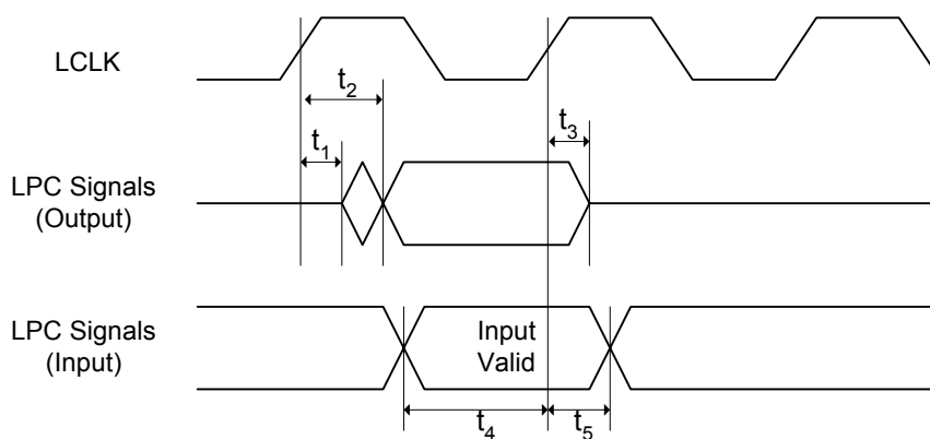
Figure 9-2. LPC Waveform
