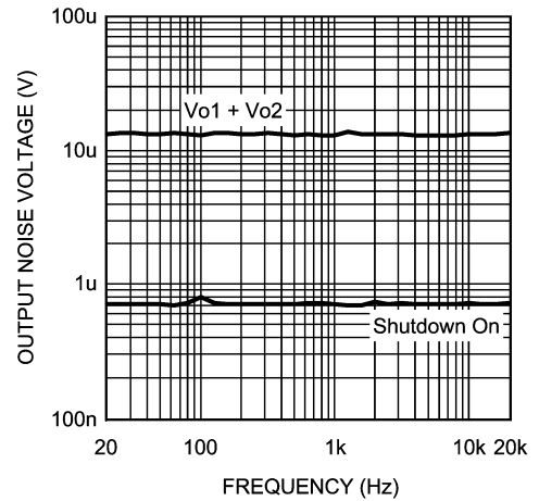
Noise Floor
