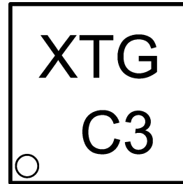
20073784 X - Date Code T - Die Run Traceability G - Boomer Family C3 - LM4898ITLX
