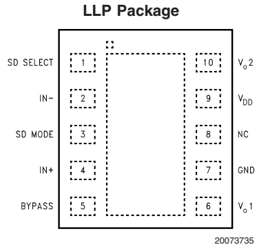
Top View Order Number LM4898LD See NS Package Number LDA10B
