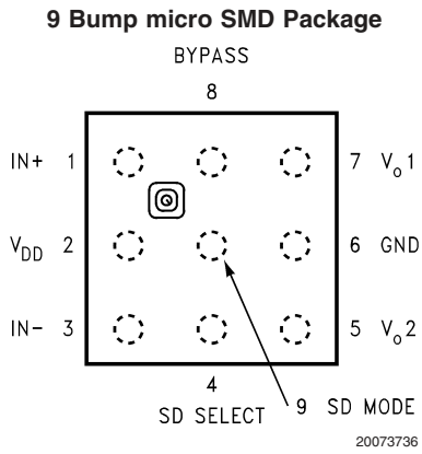
Top View Order Number LM4898ITL, LM4898ITLX See NS Package Number TLA09AAA
