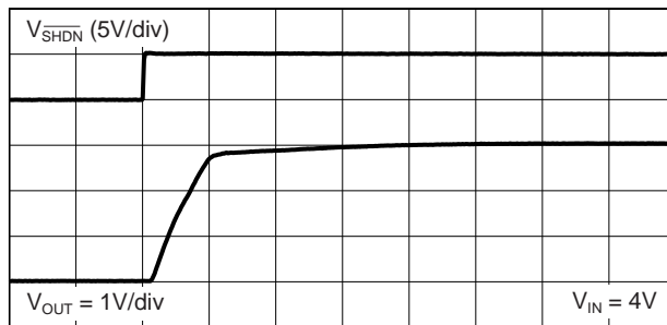
Turn-On Time From Enable ( V_{IN} present) ( C_{BYP} = 10nF )
