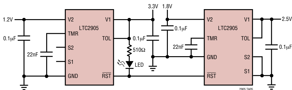
Quad Supply Monitor with LED Undervoltage Indicator, 5% Tolerance, 3.3V, 2.5V, 1.8V, 1.2V
