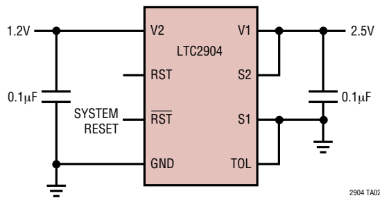
2.5V, 1.2V Supply Monitor, 10% Tolerance
