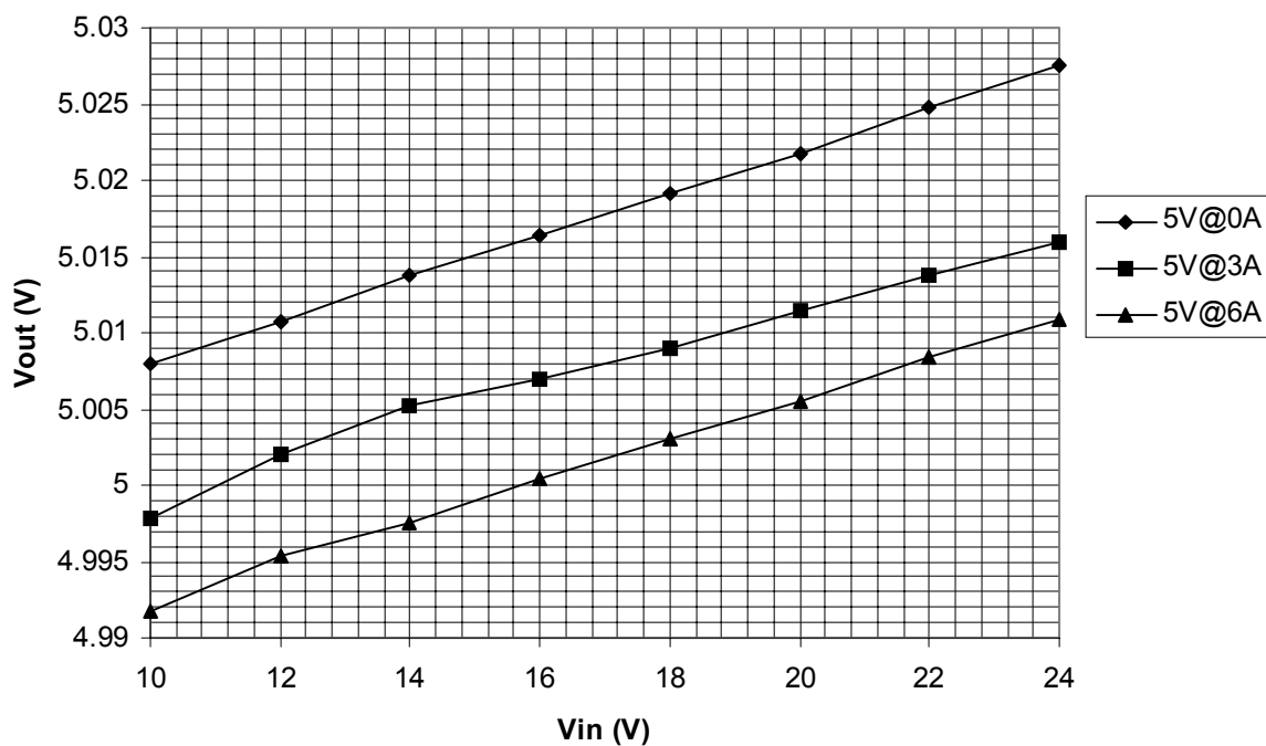
5V Line Regulation
