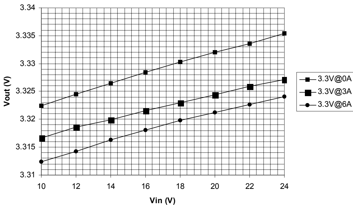
3.3V Line Regulation
