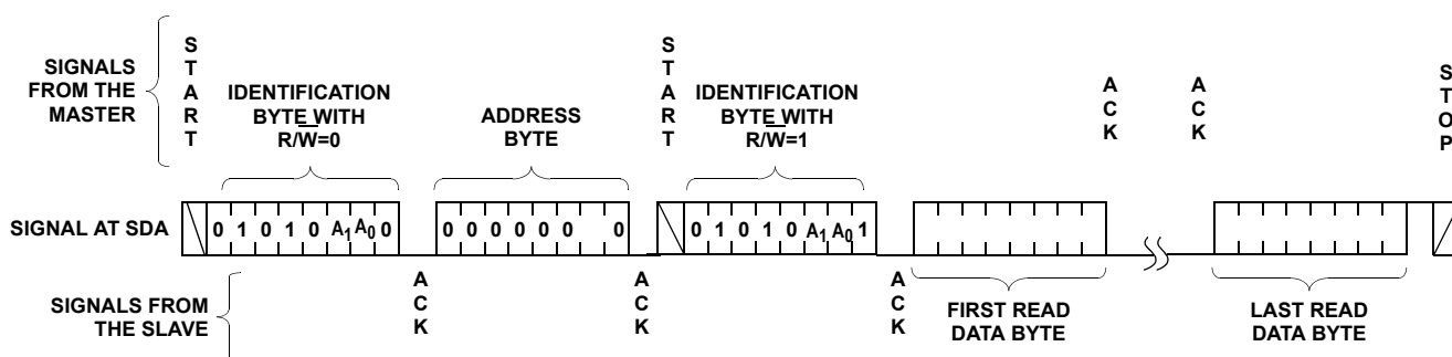
FIGURE 4. READ SEQUENCE
