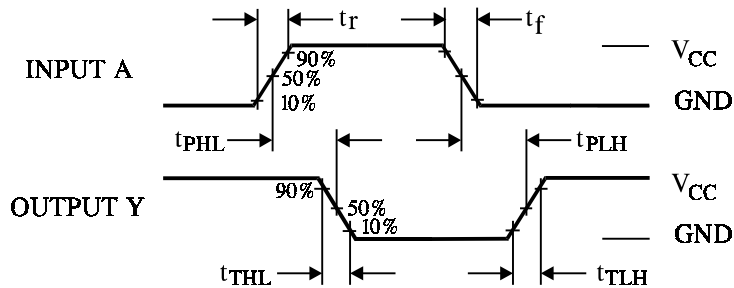
Figure 1. Switching Waveforms
