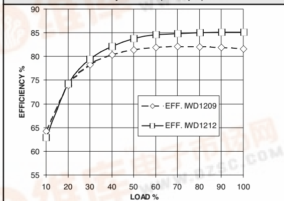
Efficiency vs. Load (12V Input)
