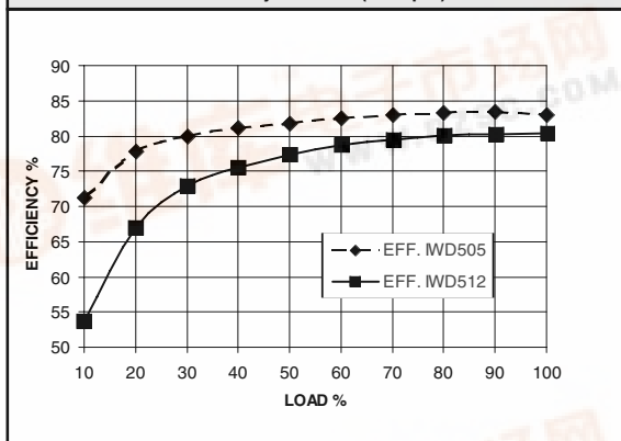
Efficiency vs. Load (5V Input)
