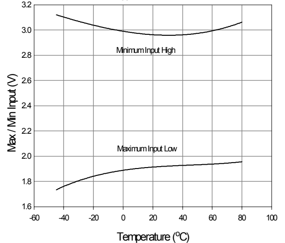
Fig. 8 Max / Min Input vs. Temperature V_{OC}=18V C_L=1nF
