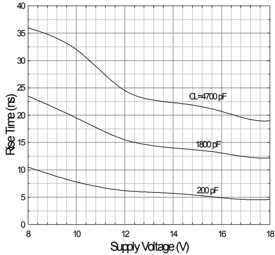
Fig. 3 Rise Time vs. Supply Voltage
