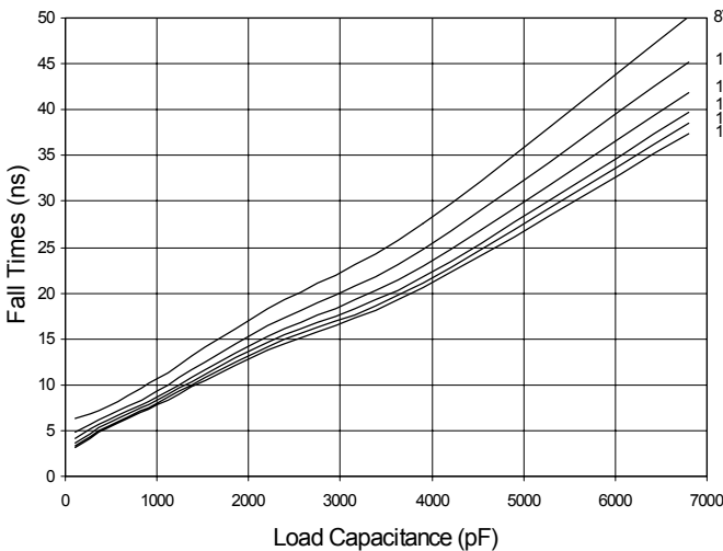
Fig. 7 Output Fall Times vs. Load Capacitance
