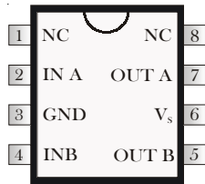
8 Lead PDIP (PI) 8 Pin SOIC (SI) IXDN402
