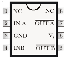
8 Lead PDIP (PI) 8 Pin SOIC (SI) IXDI402
