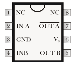
8 Lead PDIP (PI) 8 Pin SOIC (SI) IXDF402
