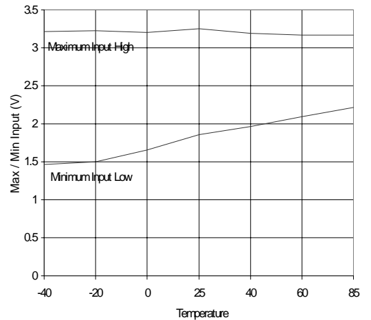
Fig. 8 Max/Mn Input vs. Temperature
