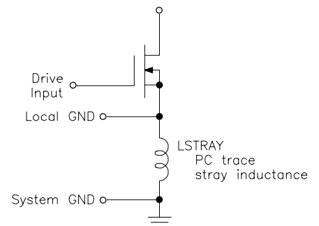
Fig. 6. Power circuit noise generation
