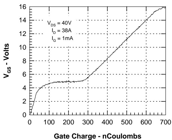
Figure 7. Gate Charge
