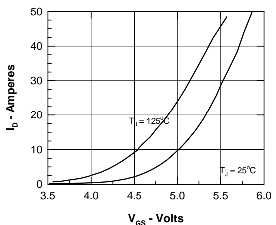
Figure 6. Admittance Curves
