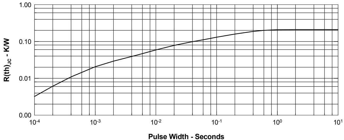
Figure 10. Transient Thermal Resistance
