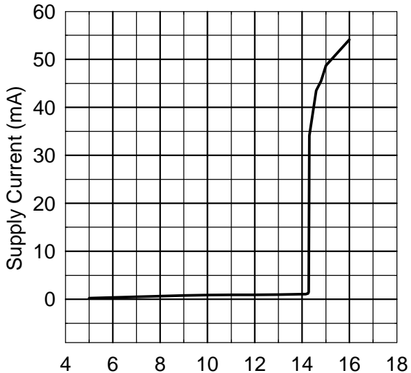
Graph 7: Supply Current vs. Shunt Voltage
