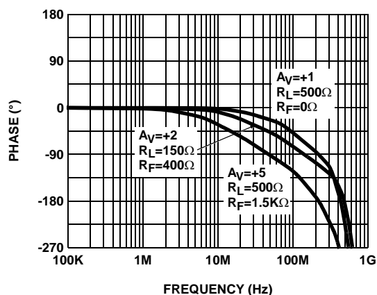
FIGURE 2. PHASE vs FREQUENCY FOR VARIOUS GAINS
