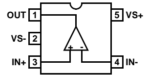
EL5151 (5-PIN SOT-23) TOP VIEW
