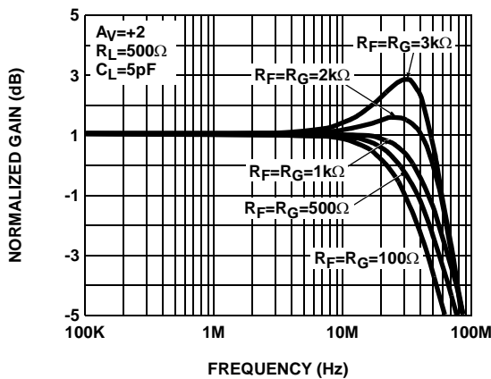
FIGURE 13. EL5150 GAIN vs FREQUENCY FOR VARIOUS R_F/R_G
