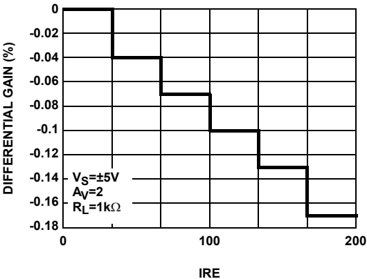
FIGURE 11. DIFFERENTIAL GAIN
