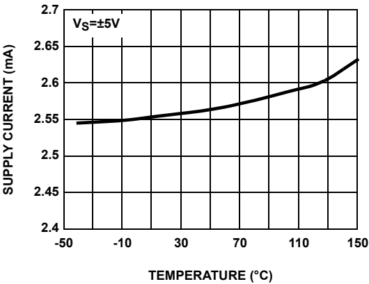
FIGURE 10. SUPPLY CURRENT PER AMPLIFIER vs TEMPERATURE
