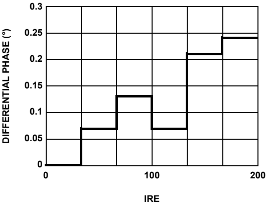
FIGURE 12. DIFFERENTIAL PHASE
