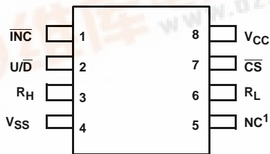
X93154 (8 LD MSOP) TOP VIEW
