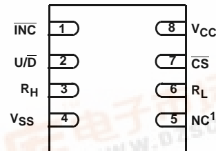
X93154 (8 LD TDFN) TOP VIEW
