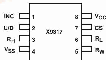
X9317 (8 LD DIP, 8 LD SOIC, 8 LD MSOP) TOP VIEW
