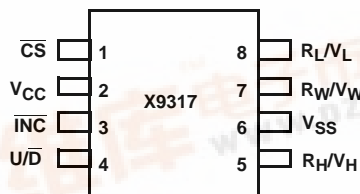
X9317 (8 LD TSSOP) TOP VIEW
