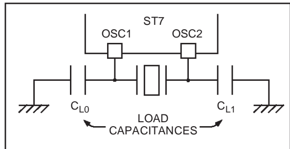
Figure 20. MO Crystal/Ceramic Resonator
