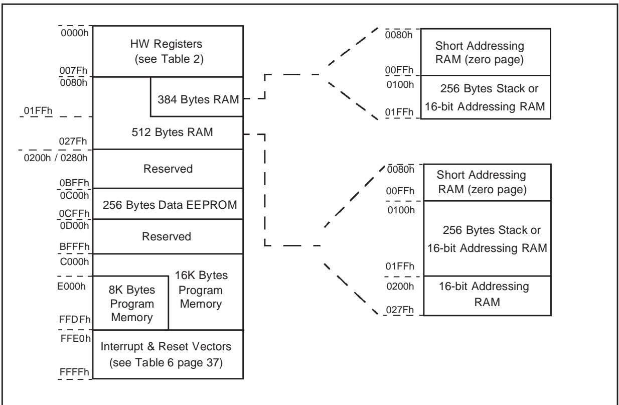
Figure 5. Memory Map
