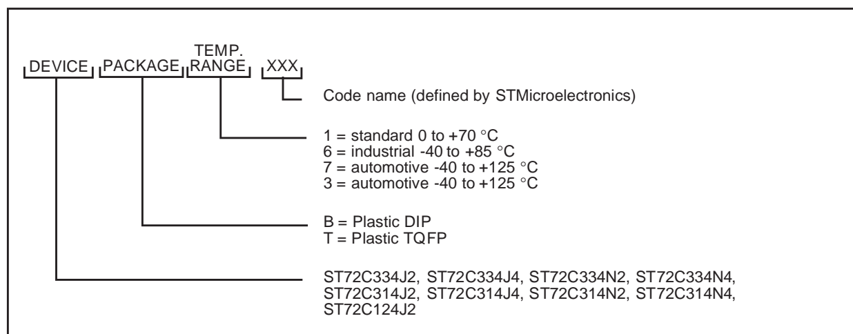
Figure 74. FLASH User Programmable Device Types
