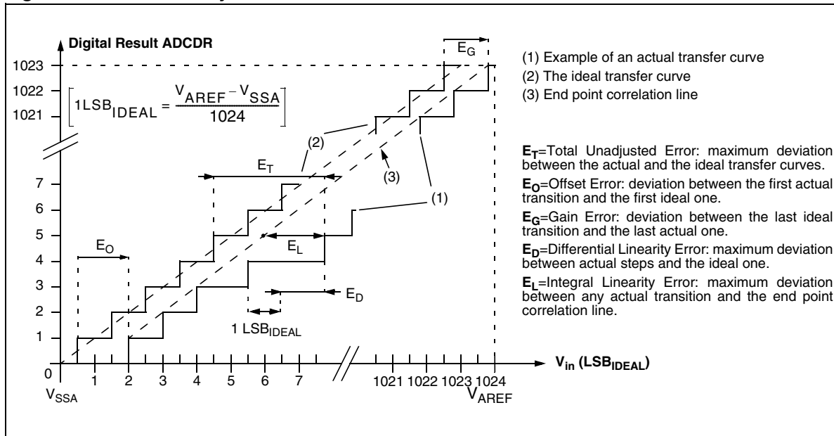
Figure 81. ADC Accuracy Characteristics
