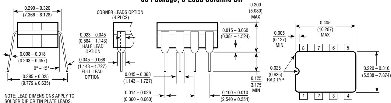
J8 Package, 8-Lead Ceramic DIP
