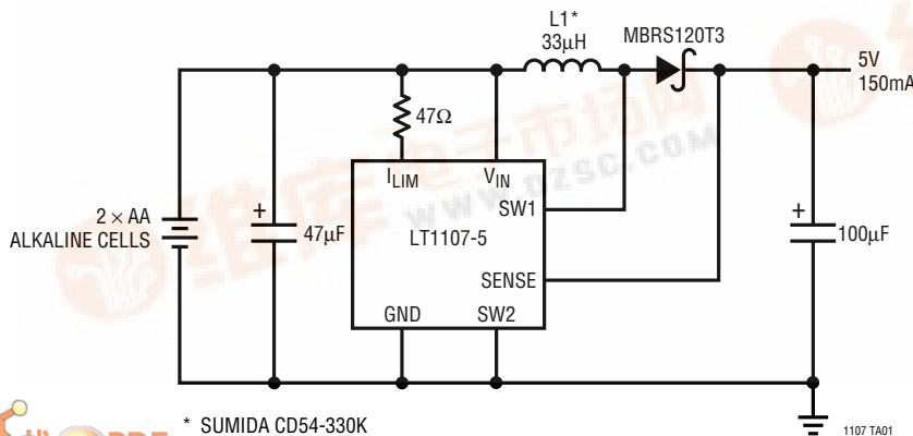
Palmtop Computer Logic Supply
