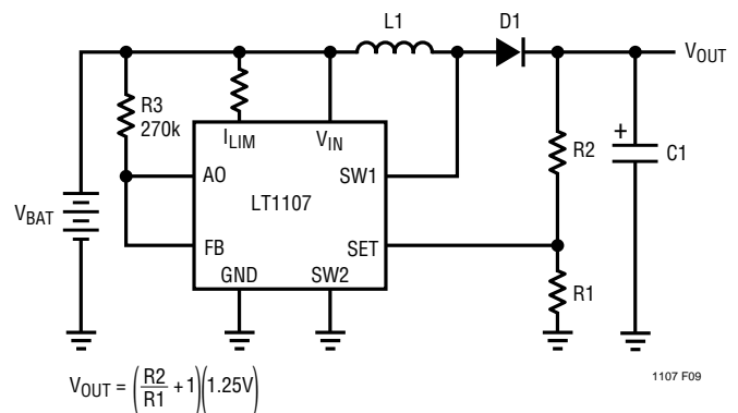
Figure 9. Output Ripple Reduction Using Gain Block
